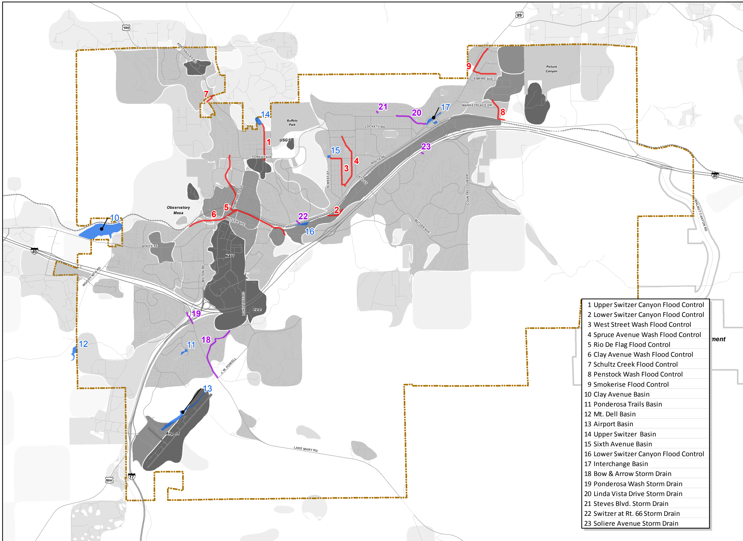
Map 11: STORMWATER FACILITIES
